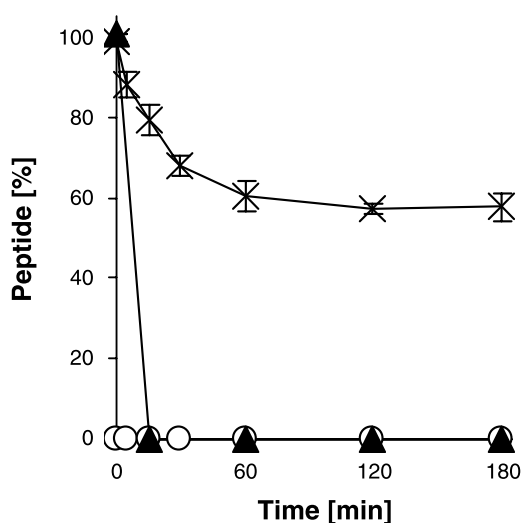
Fig. 5. Degradation of CKM and insulin by chymotrypsin (-○- SE-ET-TP-020, -×- SE-MC-TR-020, -▲- insulin); each point represents the mean \pm S.D. of at least n=3 experiments
