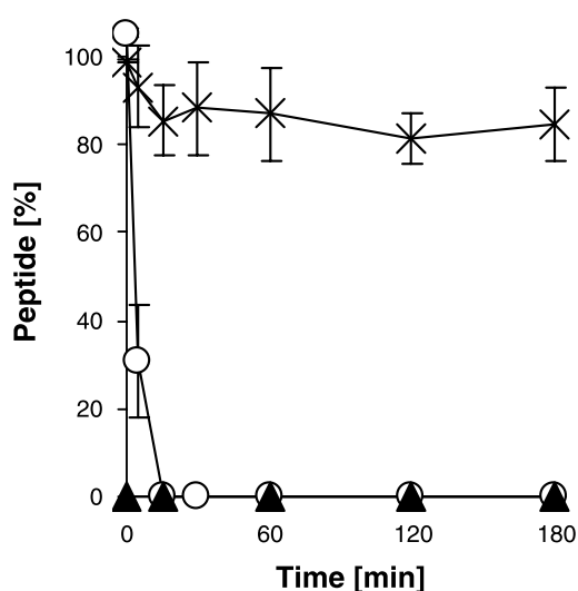
Fig. 4. Degradation of CKM and insulin by pepsin (-○- SE-ET-TP-020, -×- SE-MC-TR-020, -▲- insulin); each point represents the mean \pm S.D. of at least n=3 experiments
