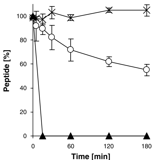
Fig. 2. Degradation of CKM and insulin by porcine gastric juice (-○- SE-ET-TP-020, -×- SE-MC-TR-020, -▲- insulin); each point represents the mean \pm S.D. of at least n=3 experiments
