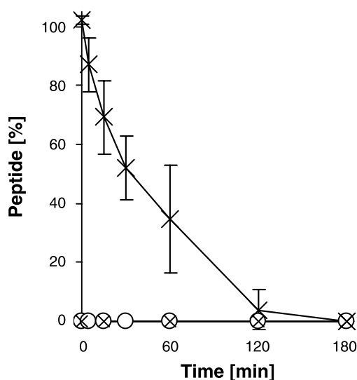
Fig. 3. Degradation of CKM and insulin by porcine small intestinal juice (-○- SE-ET-TP-020, -×- SE-MC-TR-020, ⊗ insulin); each point represents the mean \pm S.D. of at least n=3 experiments
